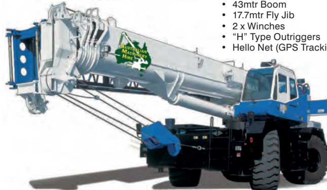
60T Rough Terrain Crane:
